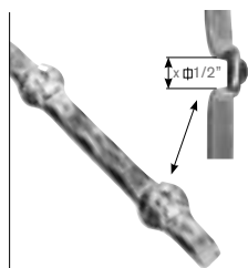
Art. 614/5 Martelado Ø 14 mm - 14 Furos dist. Furos 125 mm
